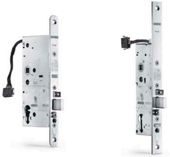
Mechanical contact lock with feedback contacts for single leaf doors
